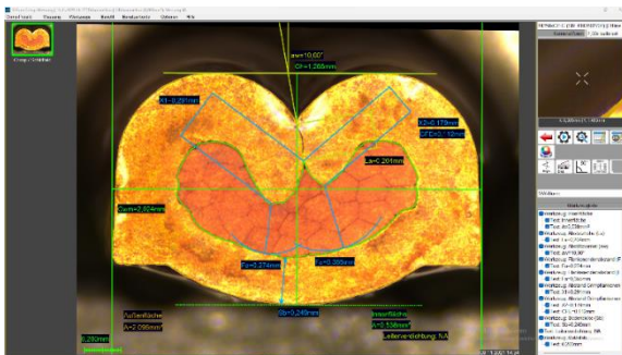
Finished microsection with X-Scan
